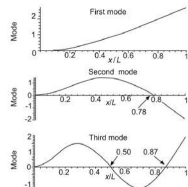
Figure 2.4: Different mode shapes of a vibrating beam.
