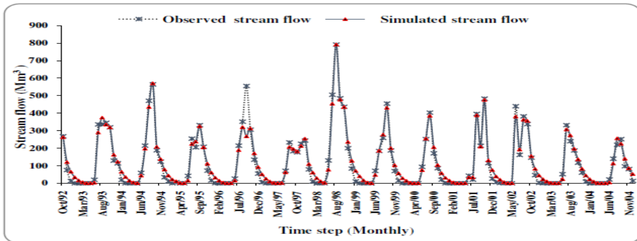
Fig. 3. Monthly observed and SWAT simulated streamflow at the Siddheswar outlet during the calibration period (1992–2004).
