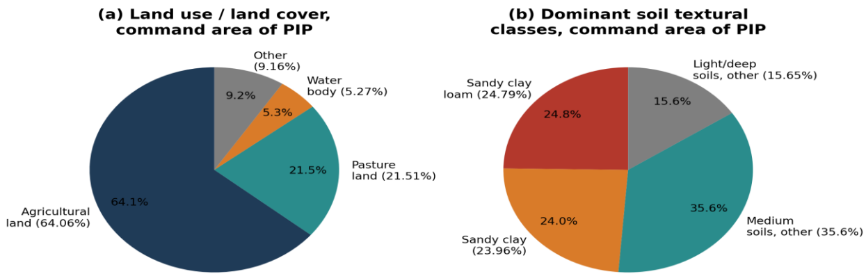
Fig. 1. (a) Land use/land cover and (b) dominant soil textural classes of the Purna Irrigation Project command area.
