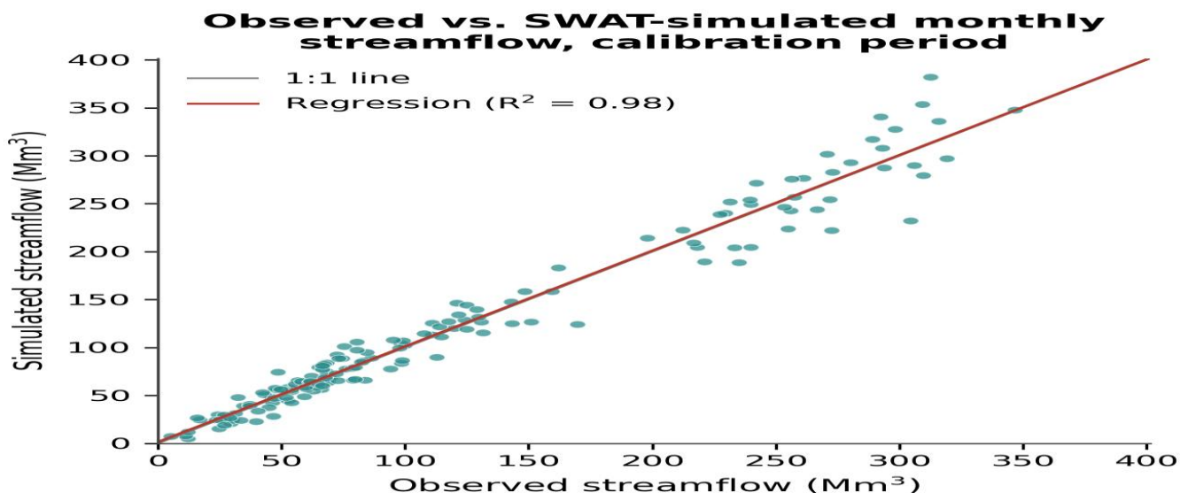
Fig. 3. Monthly observed and SWAT simulated streamflow at the Siddheswar outlet during the calibration period (1992–2004).
