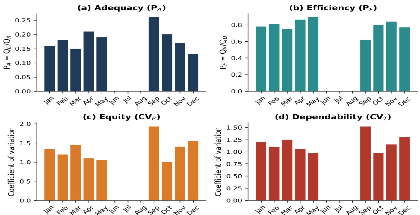
Fig. 6. Temporal variation of (a) adequacy, (b) efficiency, (c) equity and (d) dependability indicators for the Basmat branch canal, Limbgaon sub-division of PIP, 2013 - 14.
