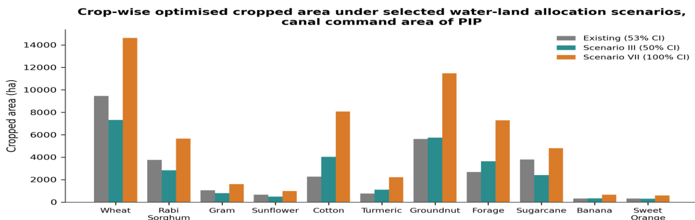
Fig. 8. Crop-wise optimised cropped area under the existing cropping pattern, Scenario III (50% cropping intensity) and Scenario VII (100% cropping intensity), canal command area of PIP.
