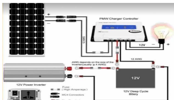
Figure 12 Wiring Diagram
