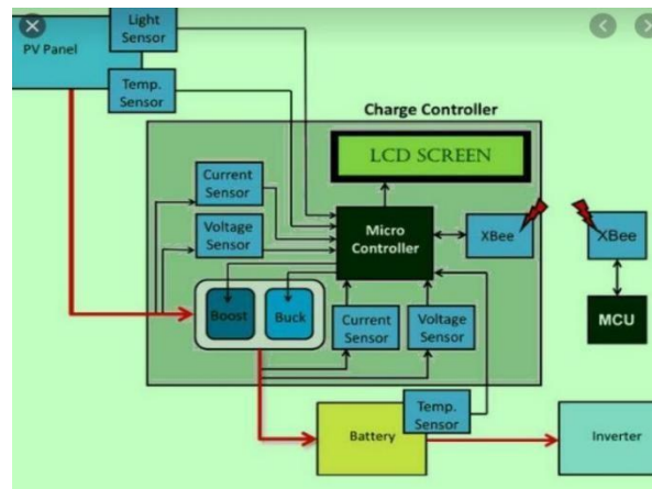
Figure 13 Micro Controller Block Diagram
