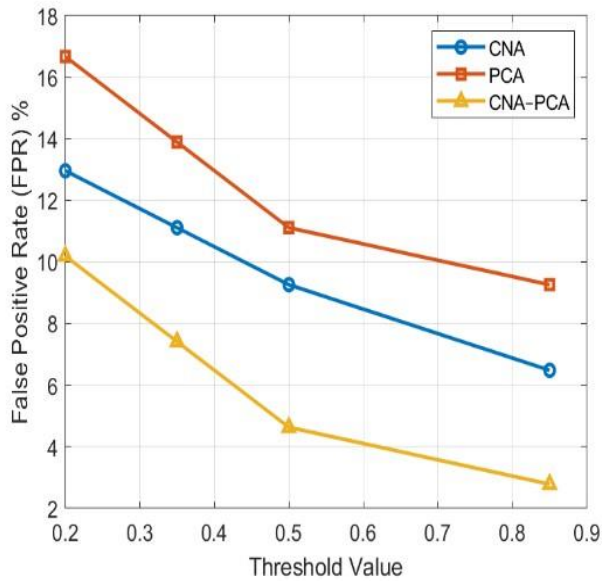
Figure 6: Graphs of FPR VS Thresholds
