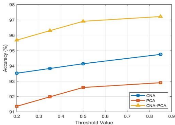
Figure 10: Graphs of Accuracy Vs Thresholds
