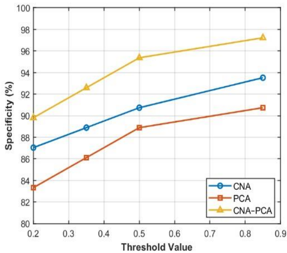
Figure 8: Graphs of Specificity Vs Thresholds
