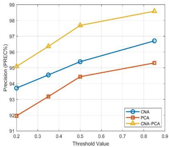
Figure 9: Graphs of Precision Vs Thresholds
