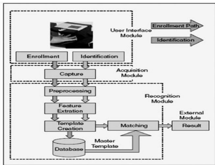
Figure 4: Architecture of the developed FFAS
