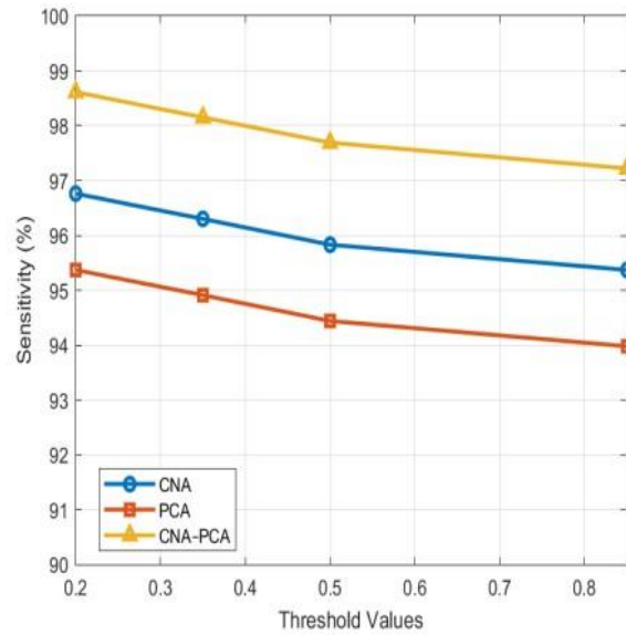
Figure 7: Graphs of Sensitivity Vs Thresholds
