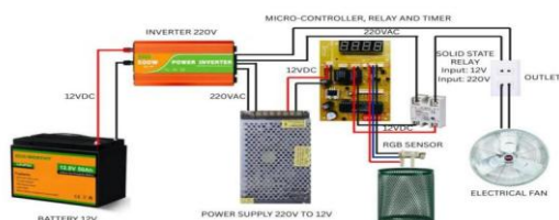
Figure 1 System Diagram of the Plastic Bottle-Activated Fan Prototype
