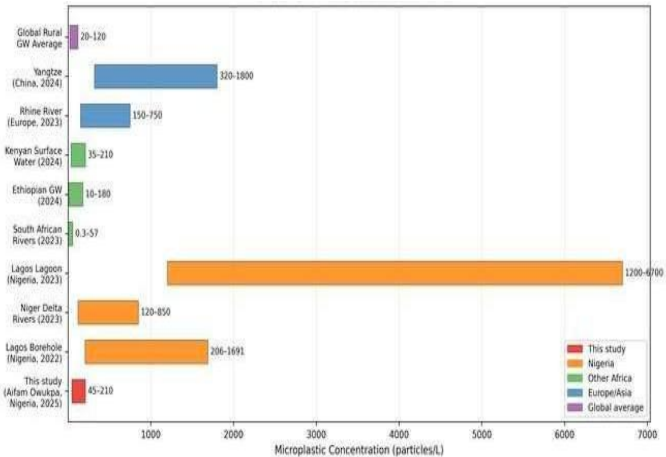
Figure 10. Horizontal bar chart comparing MP concentration ranges (particles/L) reported in this study (Aifam Owukpa, 2025) with published values from African and global freshwater and groundwater studies. Bar widths represent the reported concentration range; colour coding distinguishes geographic origin.
