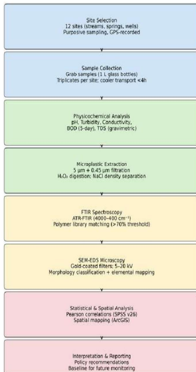
Figure 1. Schematic Flowchart of Analytical Methodology for MP/NP Detection in Water Sources of Aifam Owukpa
