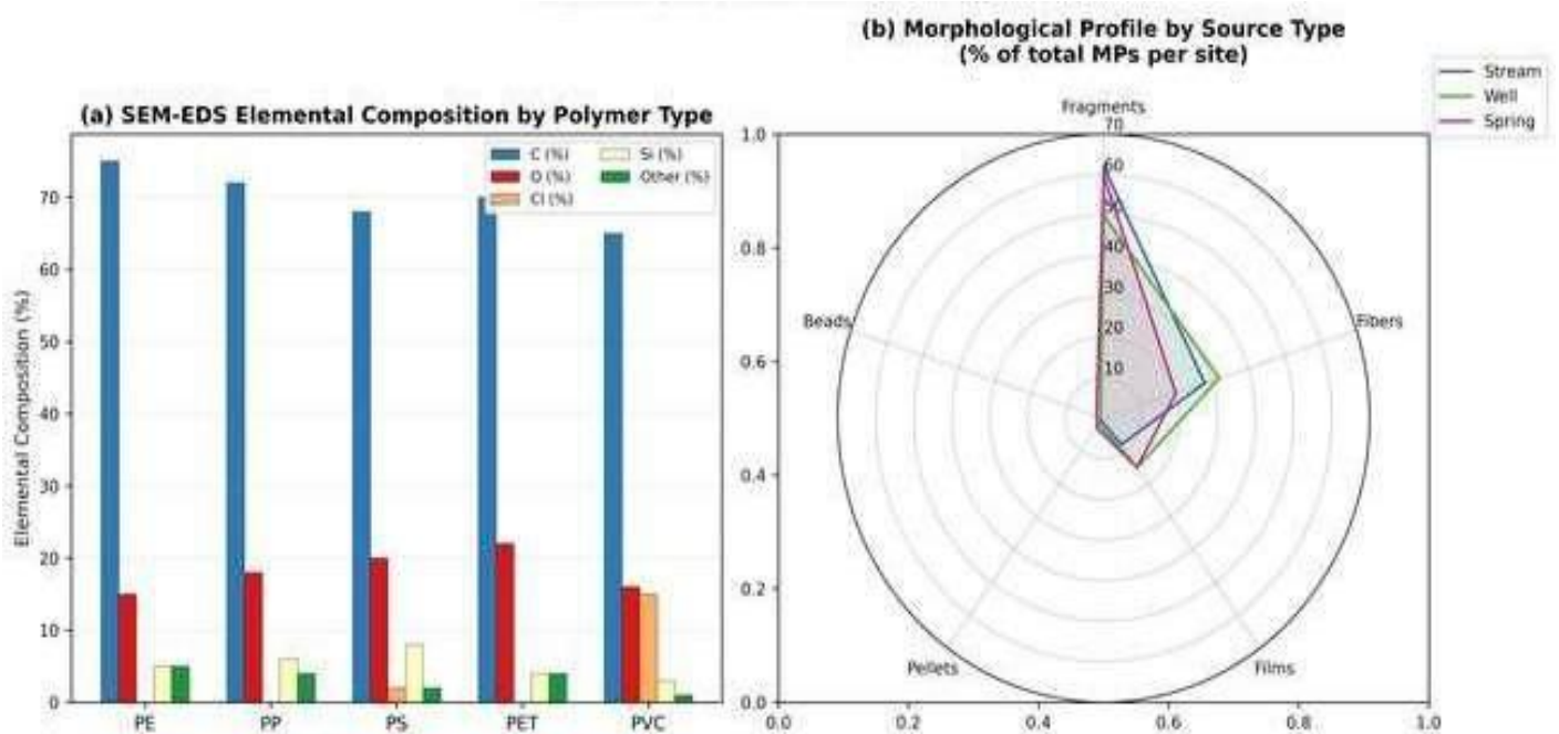
Figure 9. (a) Grouped bar chart of SEM-EDS elemental composition (C, O, Cl, Si, other) by polymer type (PE, PP, PS, PET, PVC). PVC is distinguished by the presence of 15% Cl. (b) Radar plot of morphological profiles (fragments, fibers, films, pellets, beads) disaggregated by water source type, demonstrating the higher fragment dominance in stream samples and greater fibre prevalence in well samples.
