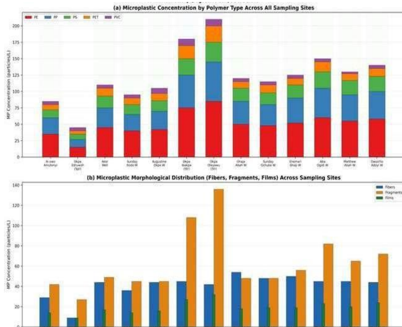
Figure 6. (a) Stacked bar chart of MP concentrations by polymer type (PE, PP, PS, PET, PVC) at all 13 sampling sites. (b) Morphological distribution (fibers, fragments, films) at each site. Stream sites (OIB, OOL) show markedly higher total concentrations and a greater fragment proportion, consistent with mechanically fragmented surface litter transported by stormwater runoff.
