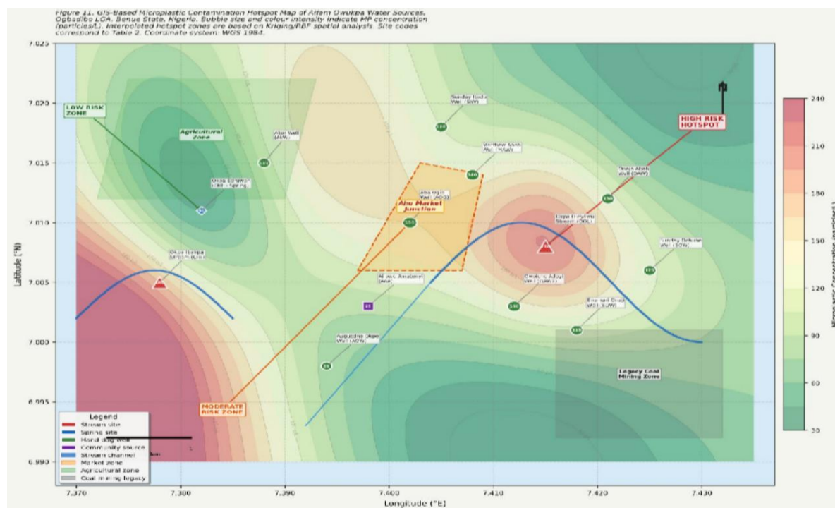
Figure 11. GIS-based microplastic contamination hotspot map of Aifam Owukpa water sources, Ogbadibo LGA, Benue State, Nigeria. Bubble size and colour intensity represent microplastic concentration (particles/L) at each sampling site. Interpolated risk zones (High Risk: >170 particles/L; Moderate Risk: 100–170 particles/L; Low Risk: <100 particles/L) are derived from radial basis function (RBF) spatial interpolation of site-measured
