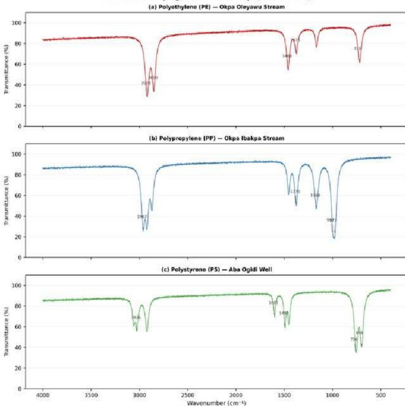
Figure 3. Representative ATR-FTIR Spectra of Identified Microplastic Polymers from Selected Sampling Sites in Aifam Owukpa (4000–400 \text{cm}^{-1} )
