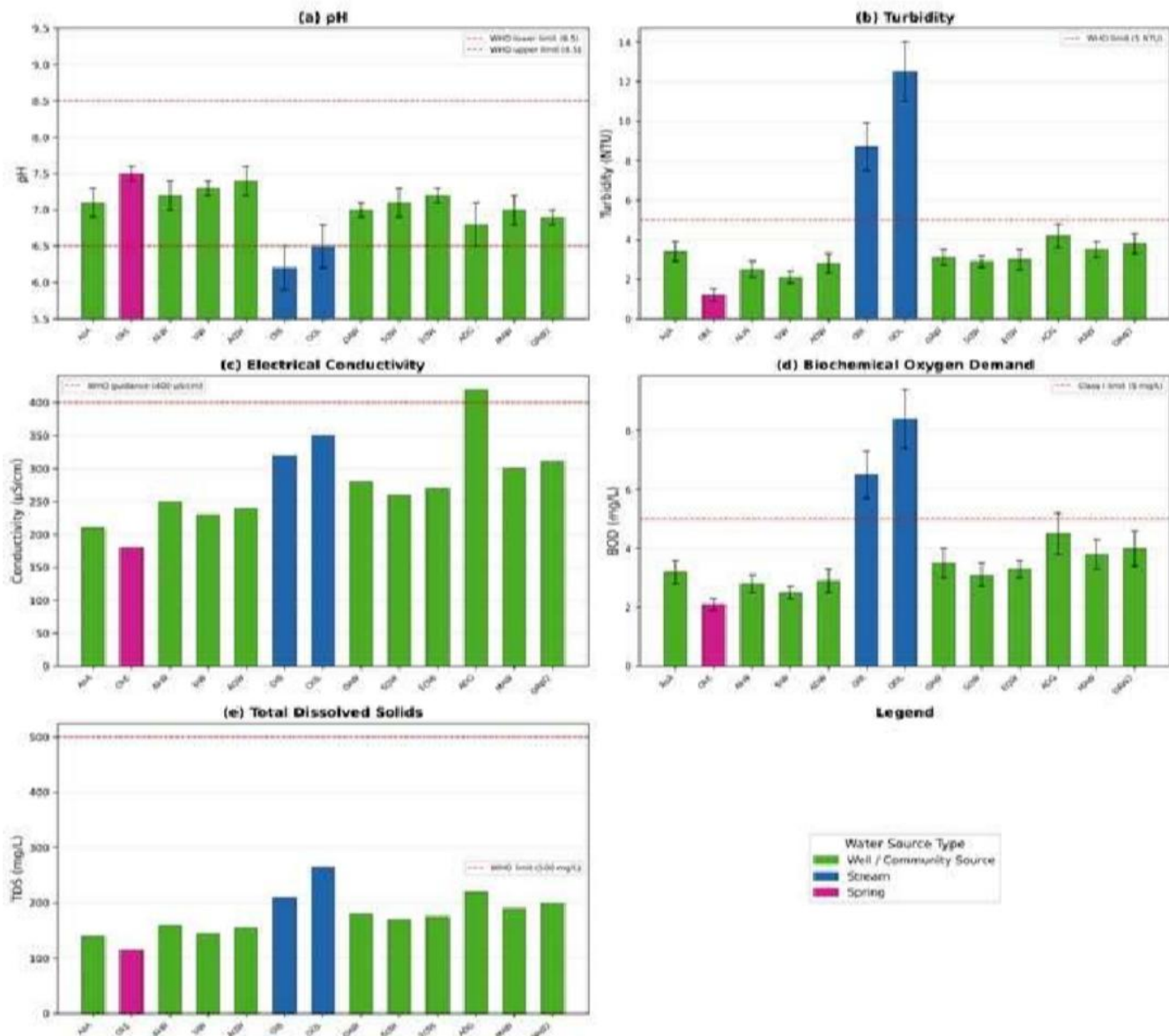
Figure 3. Multi-panel bar chart of physicochemical parameters (pH, turbidity, conductivity, BOD, TDS) across 13 sampling sites in Aifam Owukpa. Error bars represent \pm 1 SD (n = 3). Red dashed lines indicate WHO guideline threshold values. Site abbreviations: AoA = Ai owo Amutenyi; OkE = Okpa Edruwoh (spring); AkW = Akor Well; SIW = Sunday Itodo Well; AOW = Augustine Okpe Well; OIB = Okpa Ibakpa (stream); OOL = Okpa Oleyawu (stream); OAW = Onaja Abah Well; SOW = Sunday Ochube Well; EOW = Enemari Onaji Well; AOG = Aba Ogidi Well; MAW = Matthew Abah Well; OAW2 = Owoicho Adoyi Well.
