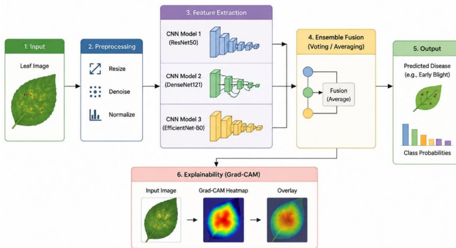
System Architecture for Plant Disease Detection
