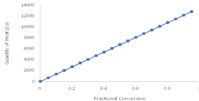
Figure 7: Profile of the PFR Quantity of Heat Generated (Q) and Fractional Conversion (X A )
