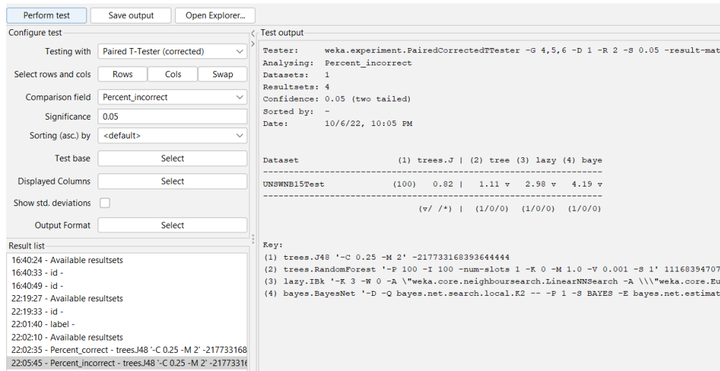
Figure 15: Percentage of incorrectly classified results.
