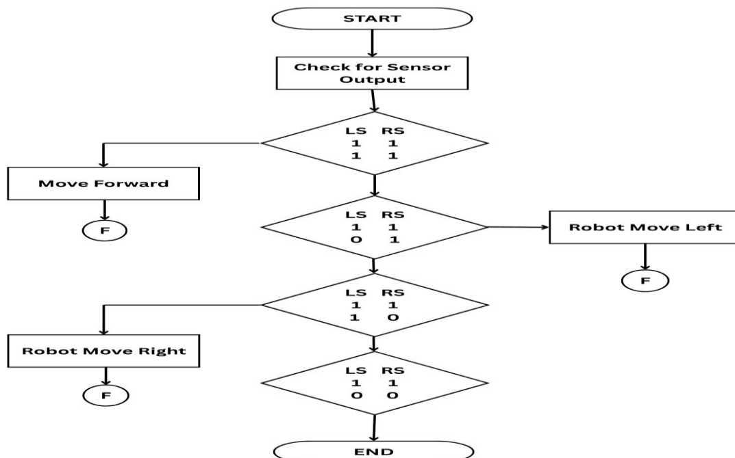
Figure 3.1.2 Flowchart for Line Follower
