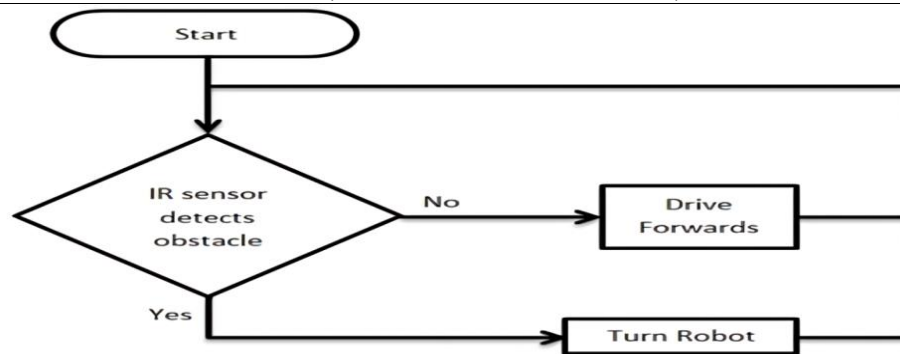
Figure 3.1.3 Flowchart for Obstacle Avoidance
