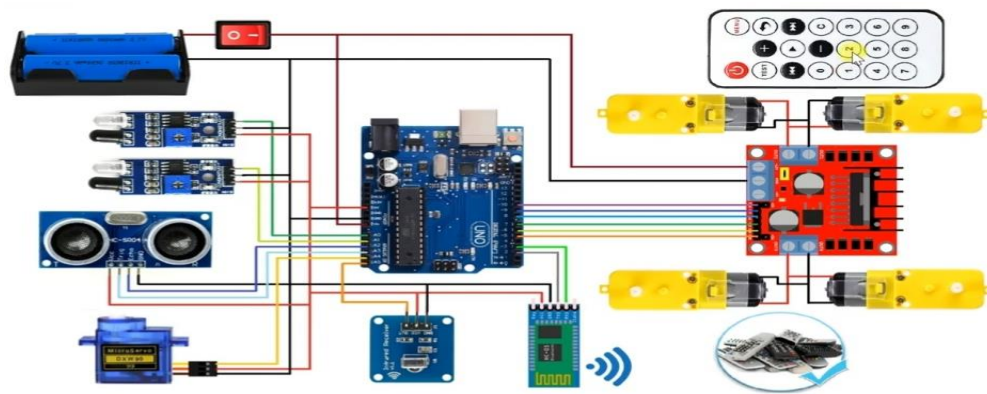
Figure 3.1.1 Schematic Diagram
