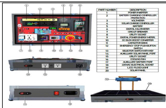
Fig. 2 Orthographic View with Major Parts of the Photovoltaic System Trainer
