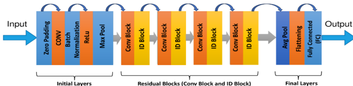
Fig. 1. Architecture of ResNet50
