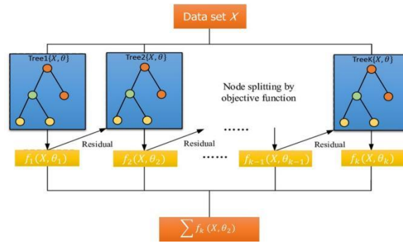
Fig. 2. Architecture of XGBoost
