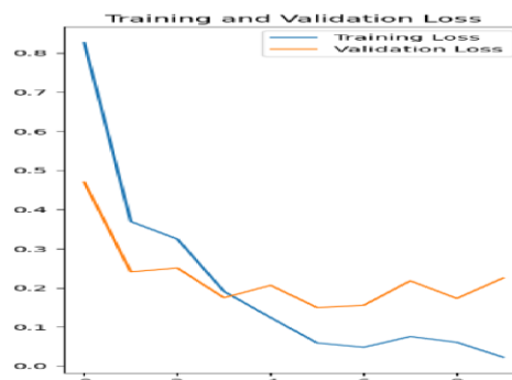
Fig. 4. Training and Validation Loss
