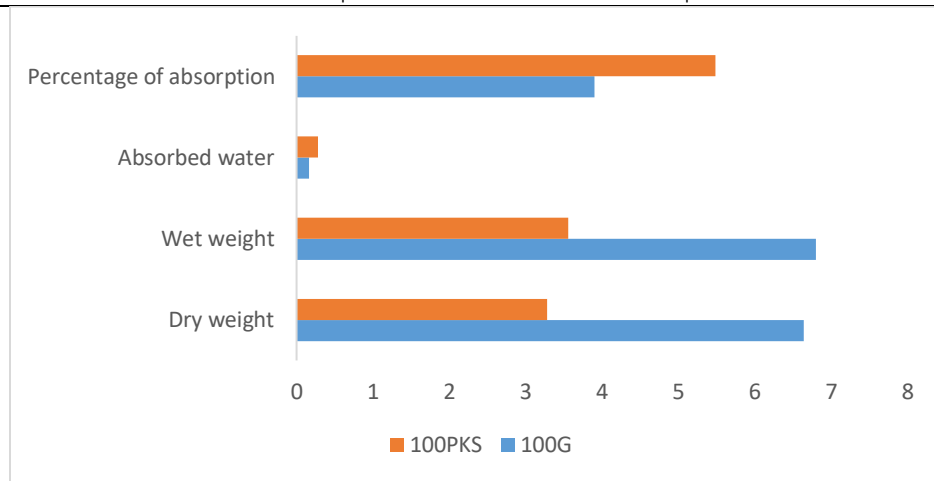
Figure 6: Absorption percentage of control mixes
