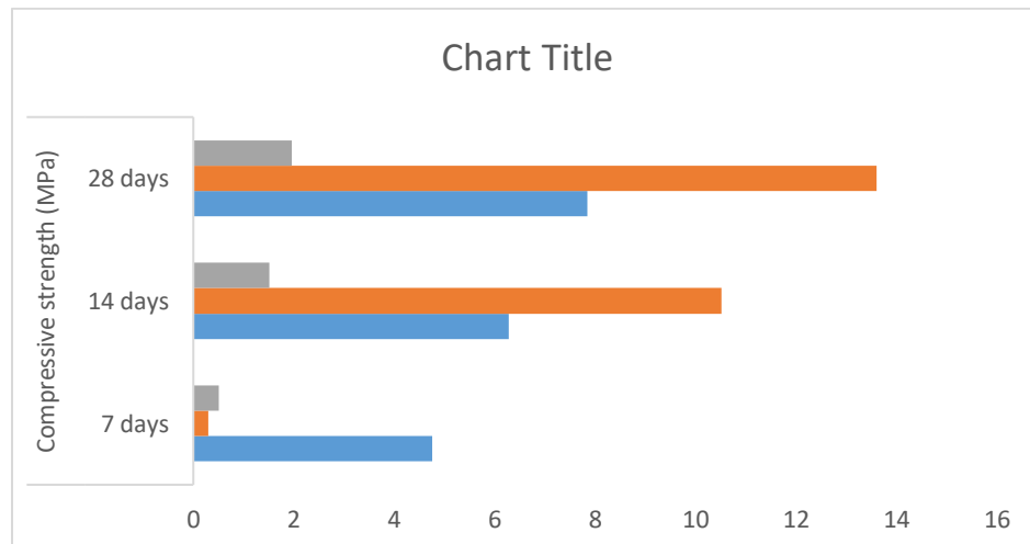
Figure 8: Compressive strength of the control
