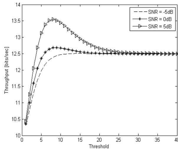
Fig. 6 Throughput vs. Threshold (SNR = -5 dB, 0 dB, 5 dB)
