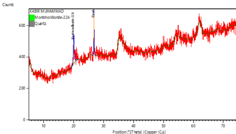
Figure 3.1 XRD result
