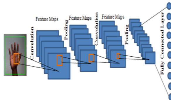
Fig.1: CNN Architecture
