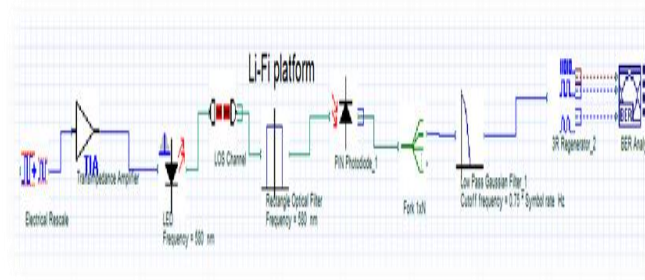
Figure 3. VLC system design in marine services platform.
