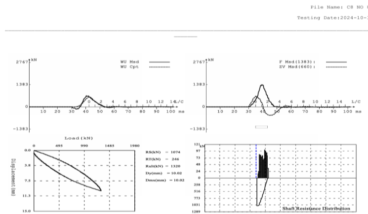
Figure 8. CAPWAP results on Pile Cap as C8 no.81
