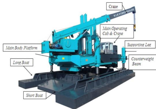
Figure 1. Hydraulic Static Pile Driver Capacity 120 Ton
