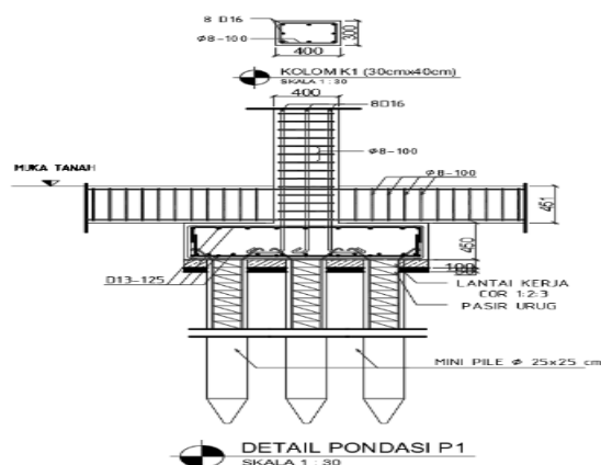
Figure 3. Pile Foundation Details
