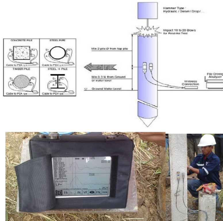
Figure 1. PDA (Case Method) and CAPWAP testing
