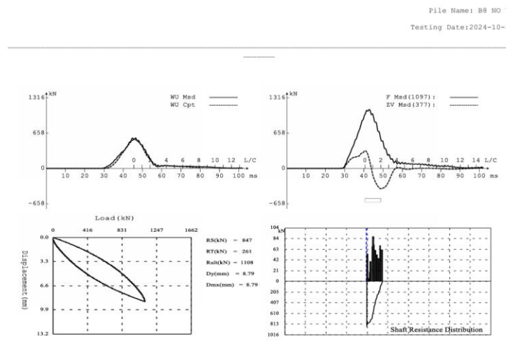
Figure 7. CAPWAP results on Pile Cap as B8 no.76
