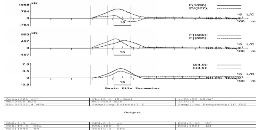
Figure 6. PDA results on Pile Cap as B8 no.76
