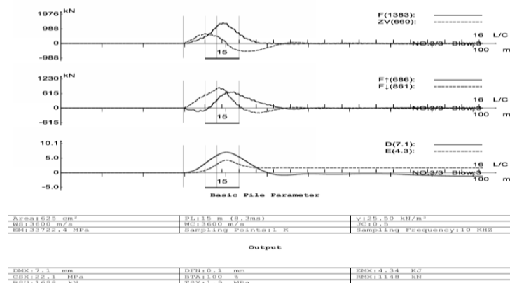
Figure 8. PDA results on Pile Cap as C8 no.81
