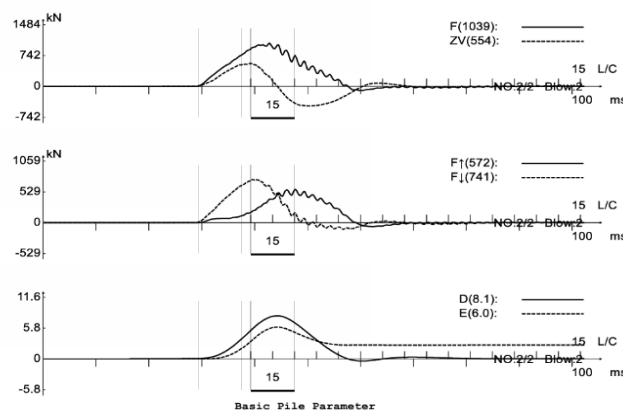
Figure 4. PDA results on Pile Cap as A8 no.71
