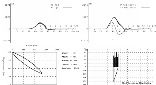
Figure 7. CAPWAP results on Pile Cap as A8 no.71
