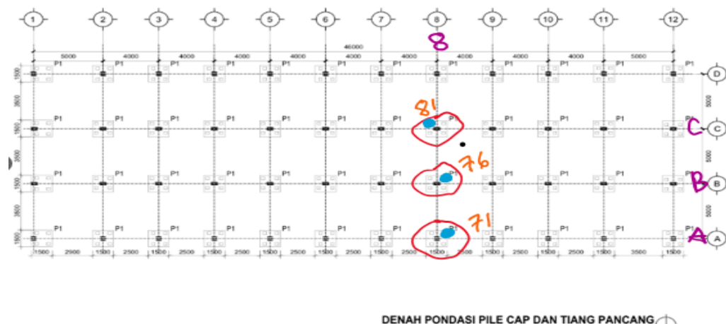
Figure 2. Pile Foundation Plan
