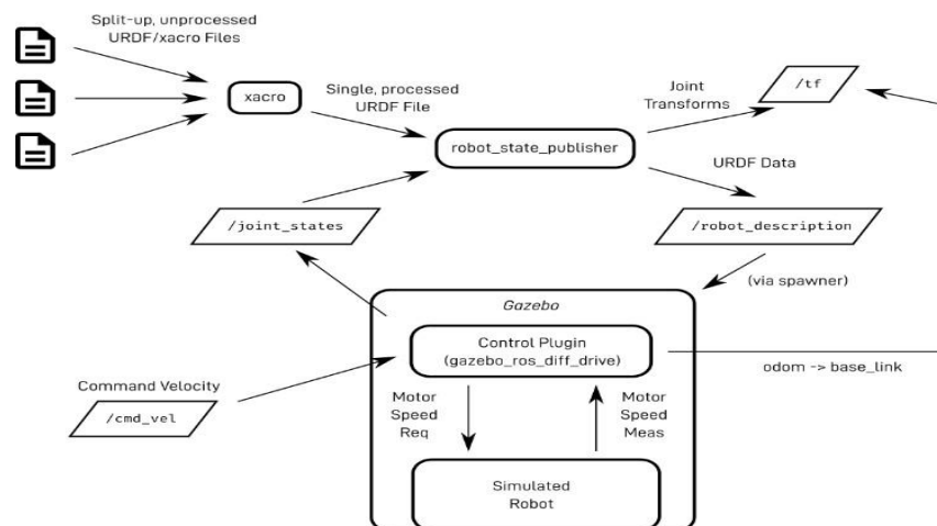
Figure 11: Robot Representation & Simulation Framework: URDF to Gazebo Control
