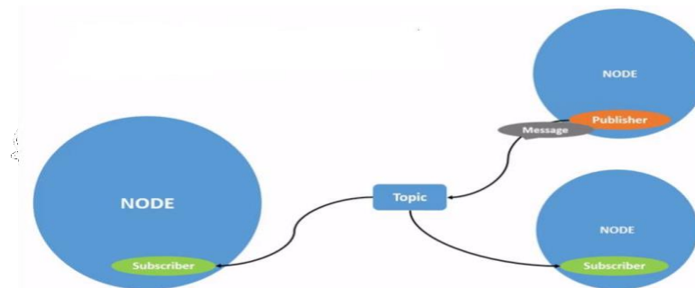
Figure 2: ROS Topic Communication between Nodes and Subscribers
