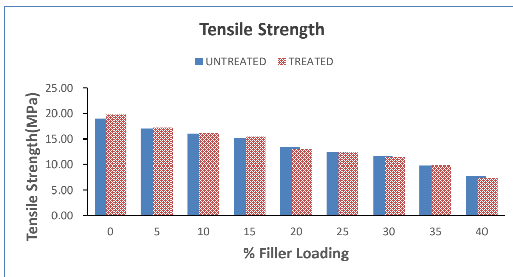
Figure 3.1. Effect of filler loading on tensile strength of treated and untreated LDPE-rattan composites.
