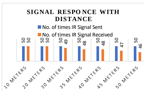
Fig. 5. The no. of times IR signal sent from transmitter vs the no. of times IR signal received to receiver chart
