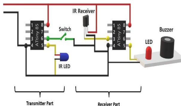
Fig. 2. Circuit diagram of the proposed system
