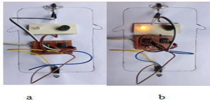
Fig. 4. (a) The full setup of the project, (b) Working scenario of the project
