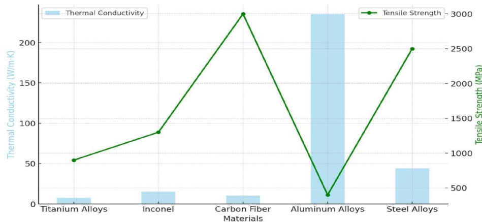
Figure 1: The trade-offs between thermal conductivity and tensile strength in materials
