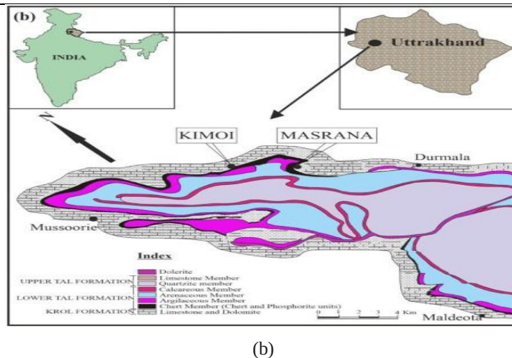
Fig. 1: (a) Map showing the distribution of the various synclines within the Krol Belt which contains Tal Group (modified after Jiang et al., 2002); (b) Geological Map showing Mussoorie location of the section examined (modified after Khan et al., 2016).
