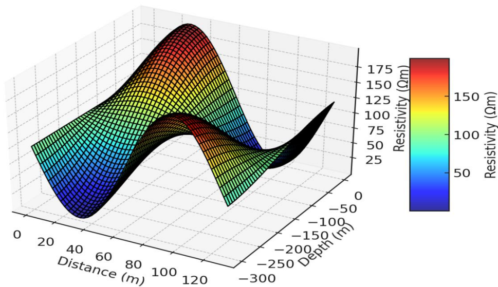
Fig:5 3D Resistivity Model profile
