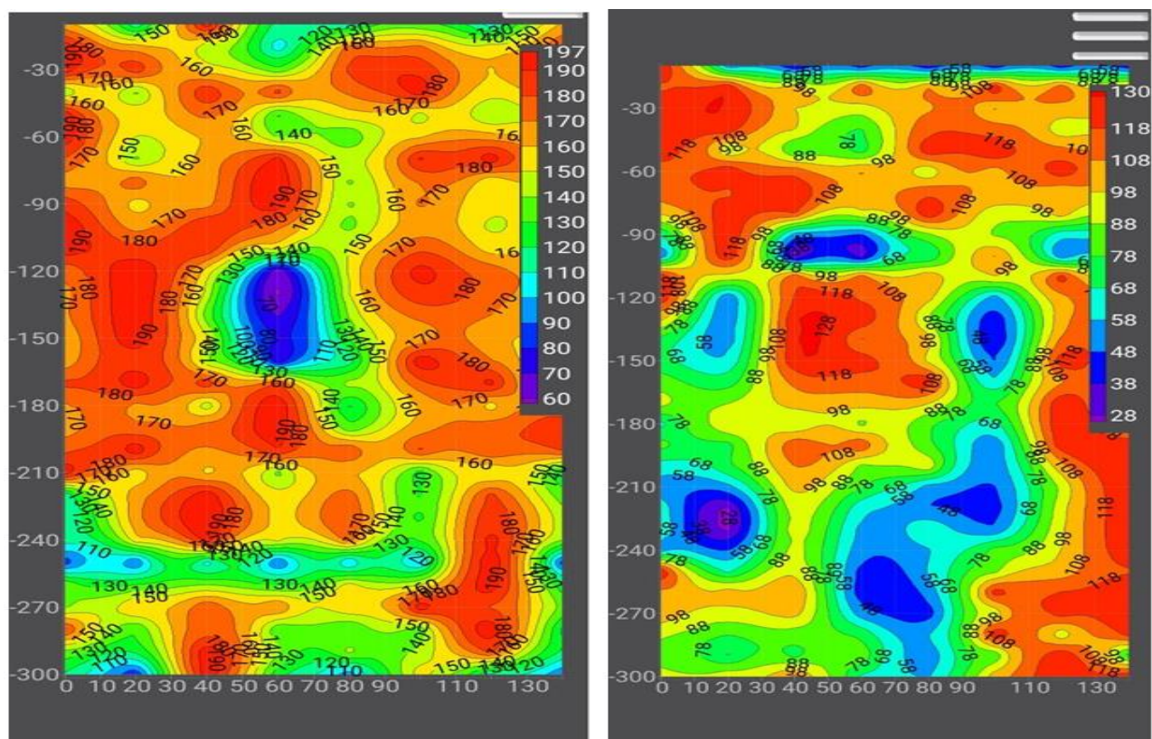
Fig :3 Magnetotelluric Profile 3&4 in the study area.
