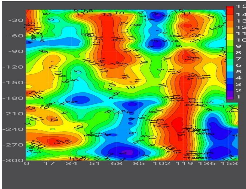
Fig :4Magnetotelluric Profile 5 in the study area.
