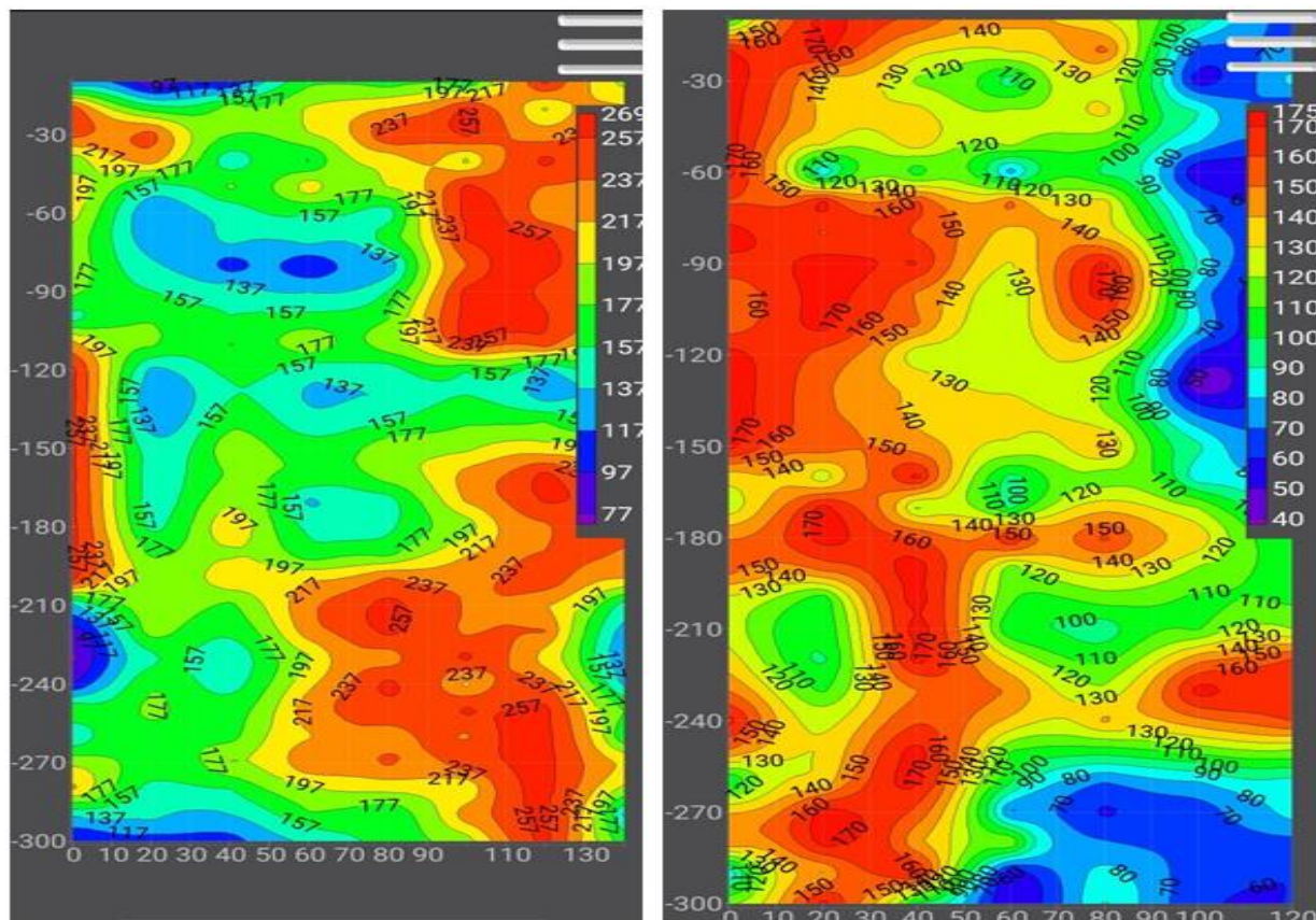
Fig:2 Magneto telluric profile 1&2 in the study Area
