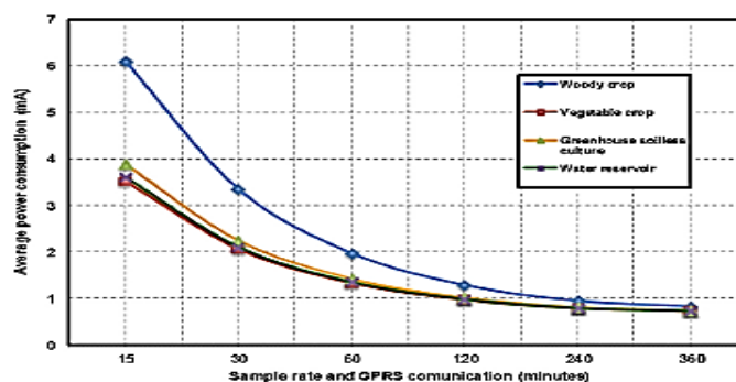
Figure 10: Graph of the average power consumption in milli-Ampere (mA) for different sample rate and time for data sent through GPRS connection, source from Figure 10 in [39]
