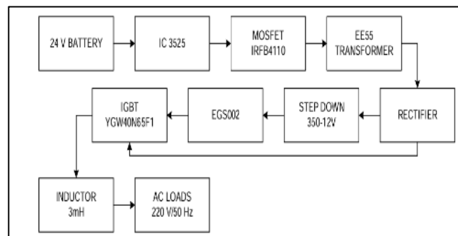
Figure 4.2.1 Block Diagram of Sine wave generation using EGS002.
