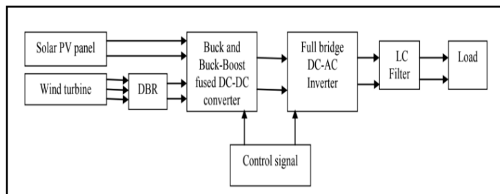
Figure 2.1 Block Diagram of multi-input inverter
