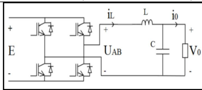
Figure 3.1 H- Bridge circuit with LC filter
