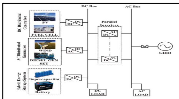
Figure 2.2 Grid-Tied HRES
