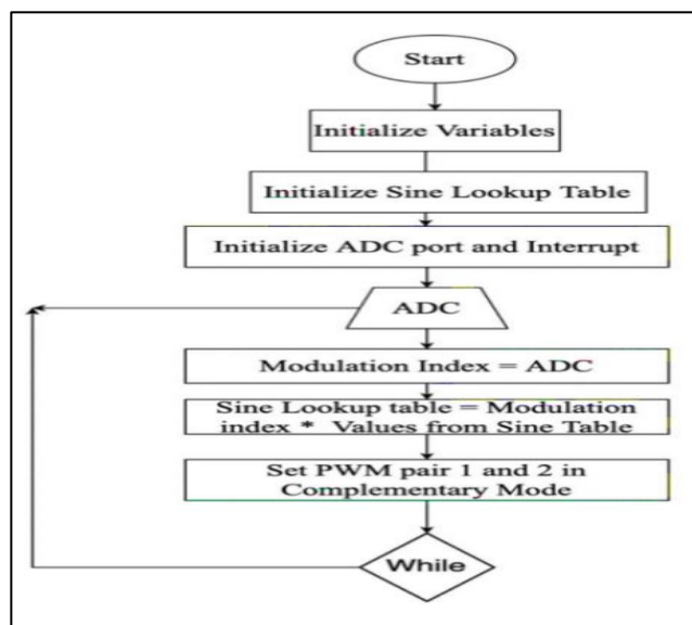
Fig 4.2.2 Program Flow of SPWM
