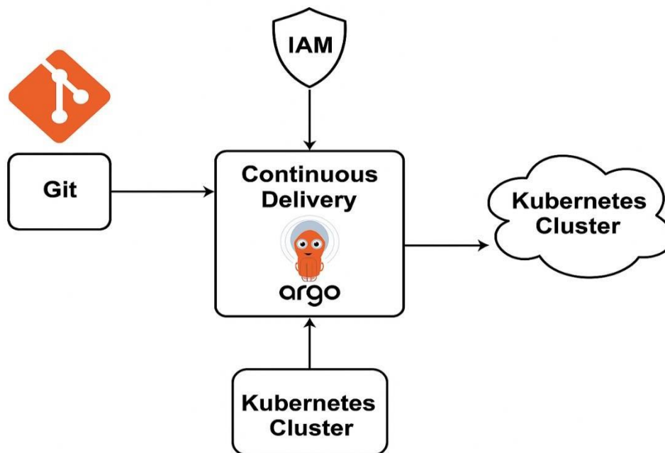
Figure 3: The combination of GitOps with ArgoCD and IAM and AWS operates as a reliable system
