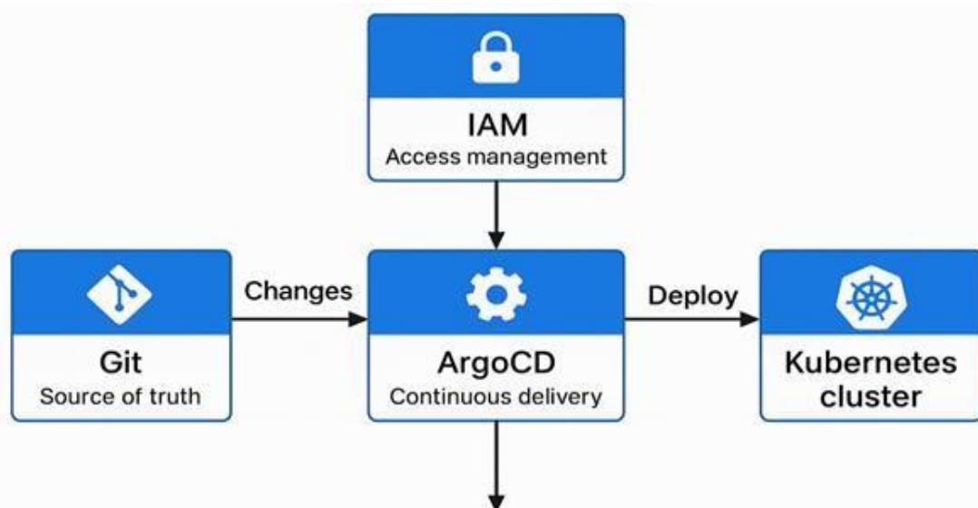
Figure 7: Demonstrates how GitOps works through iterative processes
