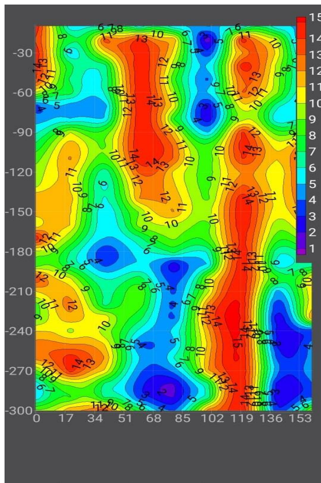
Fig :4 Magnetotelluric Profile 5 in the study area.
