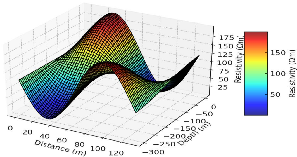
Fig: 5 3D Resistivity Model profile
