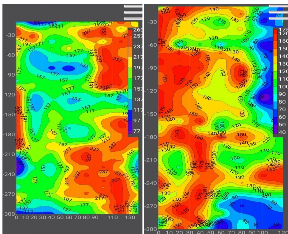
Fig:2 Magneto telluric profile 1&2 in the study Area
