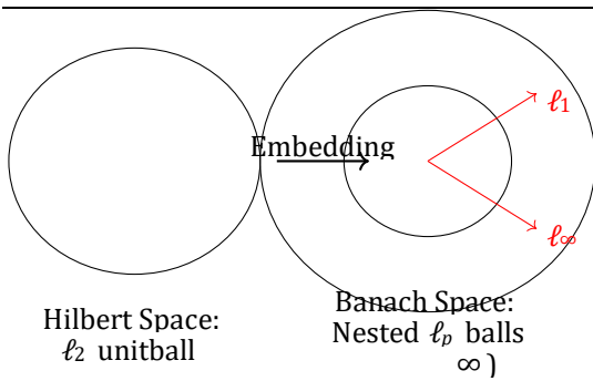
Figure 2: Geometric distinction between Hilbert (isotropic) and Banach (anisotropic) unit balls. The nested \ell_p structure enables direction-dependent regularization critical for adversarial robustness (Theorem 5). Red arrows indicate principal directions of anisotropy in Banach space.
