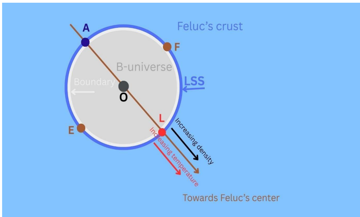
Fig.7 Position of our universe inside Feluc's crust
