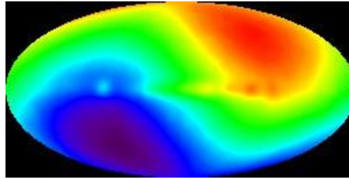
Fig.6 Warmer (red) and cooler (blue) region seen by COBE. ( NASA/JPL-Caltech)
