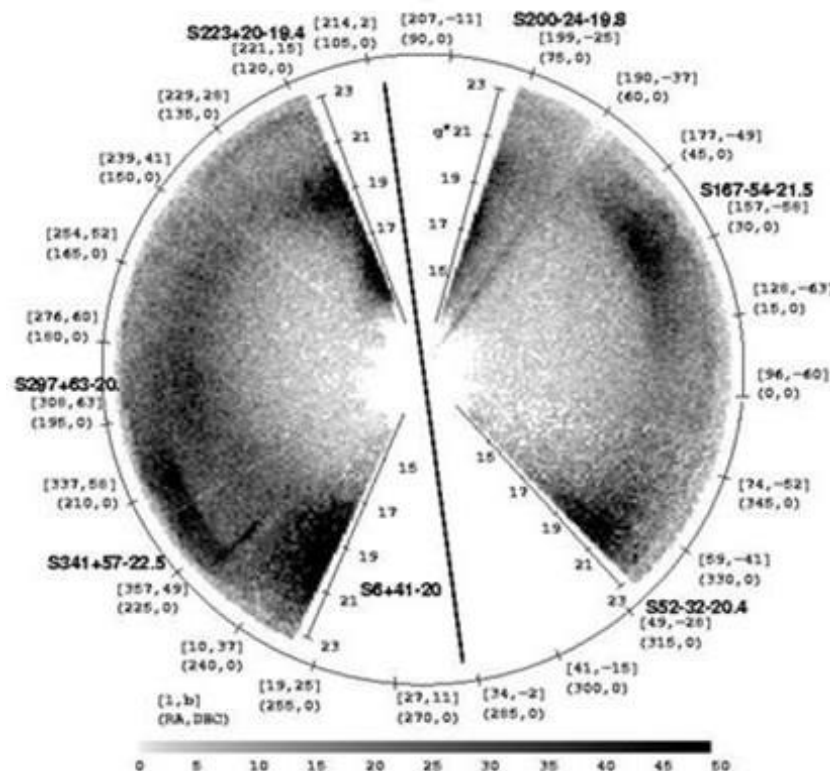
Fig.5 Blue-colored turnoff stars along celestial equator. The nearly vertical line is the celestial equator [Newberg et al. 2002]. (Reprinted by permission).
