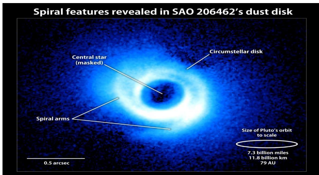
Fig. 4. SAO 206462, a young star in the constellation Lupus (NASA, 2011, http://science.nasa.gov/ ).
