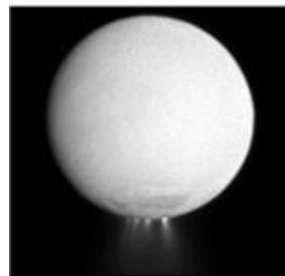
Fig.3 Plume of icy material streaming from Enceladus' south pole (NASA, 2011, http://science.nasa.gov/ )
