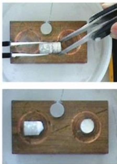
Fig. 1 The two pieces upon heating at ambient pressure, demonstrating the spatial segregation between LDA and HDA and a phase boundary in between (Winkel et al., 2011) (Reprinted by permission).
