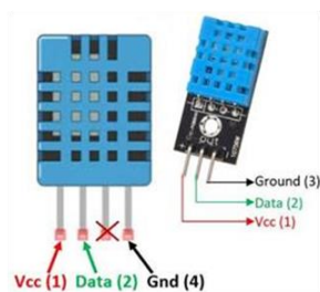
Fig. 7 DHT11 Temperature-Sensor .
