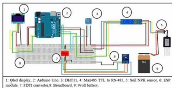
Fig. 8 Schematic diagram of the hardware components.
