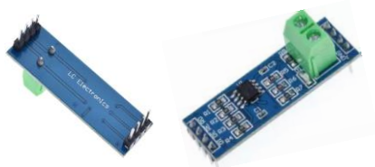
Fig. 6 MAX485 TTL to RS-485 Interface Module.
