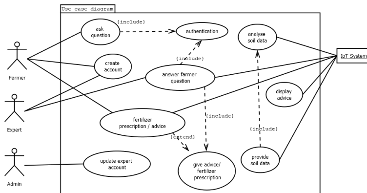
Fig. 2 The System Use Case diagram
