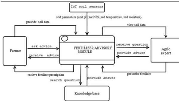
Fig. 1b The Context diagram of the system
