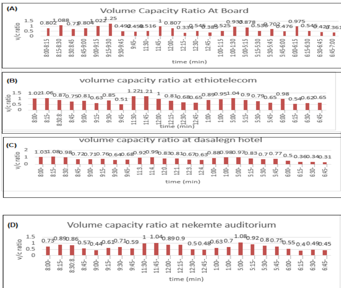
Figure 6: Volume to Capacity ratio graph at the parking area at (A) Board, (B) Ethio Telecom, (C) Dasalegn, (D) Nekemte Auditorium
