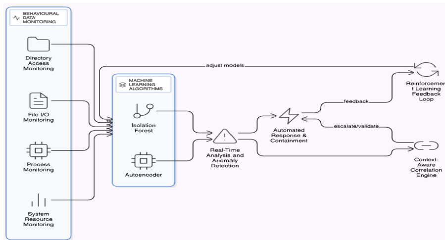
Fig. 2. AI- Enabled Threat Detection System
