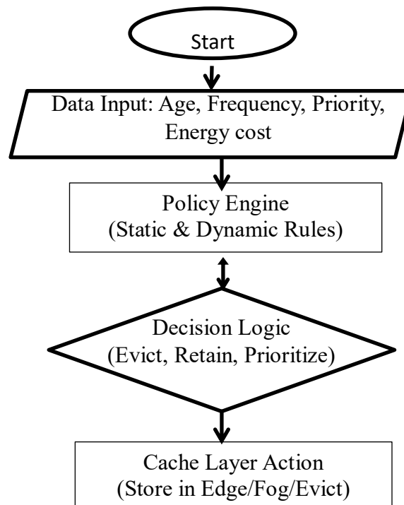
Figure 3: Flowchart showing the policy-based decision-making process based on input data characteristics and system constraints. The policy engine applies static and dynamic rules to guide cache actions such as retention, eviction or prioritization, enabling adaptive and sustainable system behaviour.
