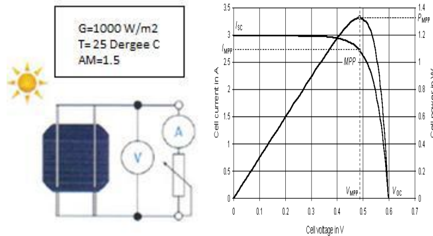
Figure 1: Current-voltage and power-voltage solar cell characteristics
