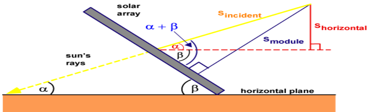
Figure 2: Solar Incidence on a plane
