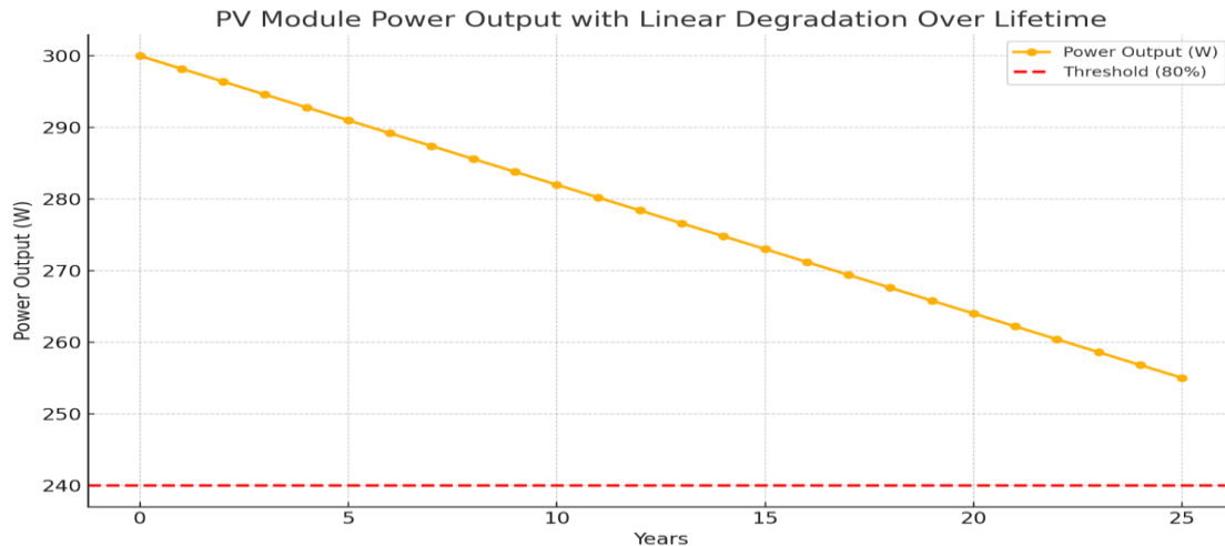
Figure 3: PV power output with linear degradation
