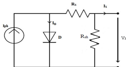
Figure 3: Electrical Equivalent Circuit model of single diode SPV module
