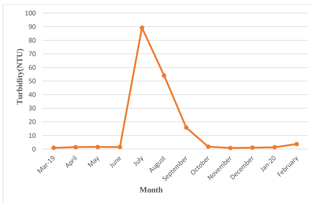
Figure 1: Monthly turbidity concentration at Amritpur (site I).
