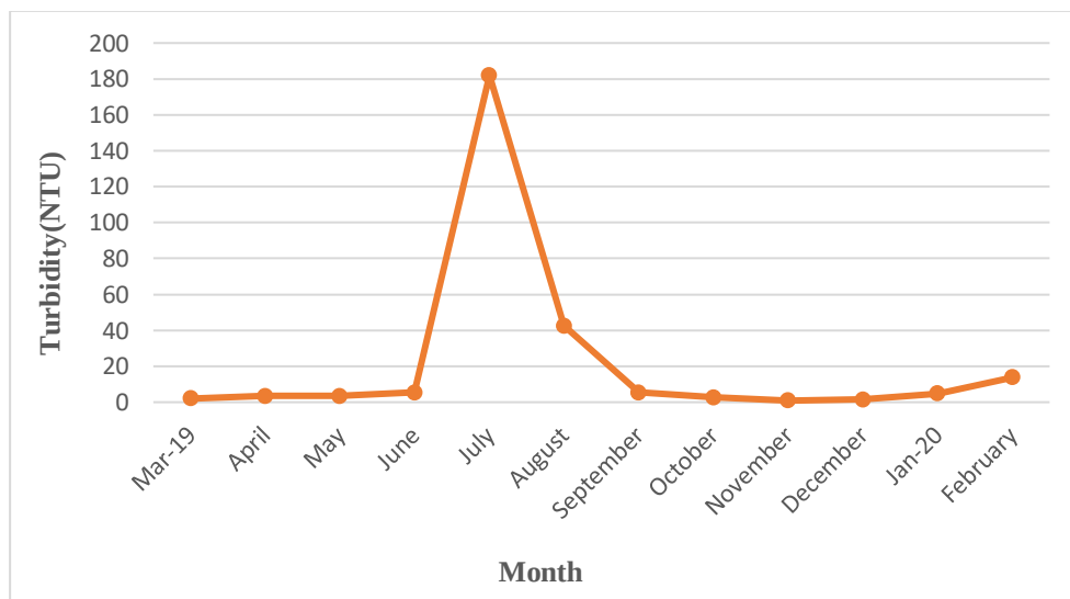
Figure 3: Monthly turbidity concentration at Kathgodam (site III)
