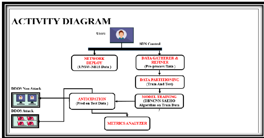
Fig 3.5 Activity diagram
