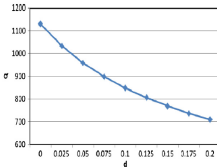
Fig. 3. Production lot size, Q vs. d .
