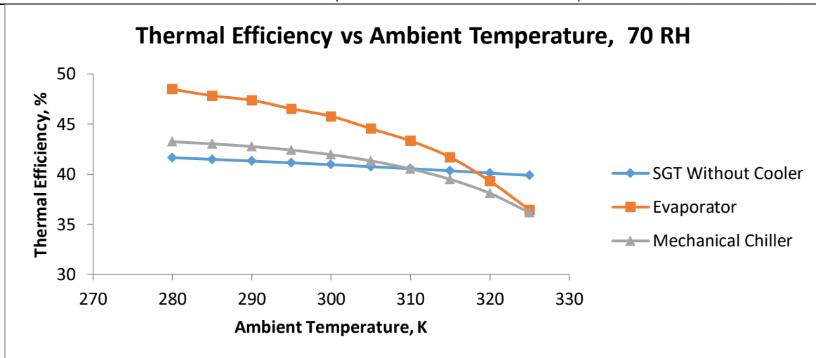
Figure 3.4- Graph of Thermal Efficiency versus Ambient Temperature, RH = 70%
