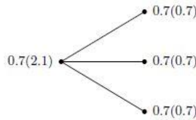
Fig. 1: FL Labeled K_{1,3}
