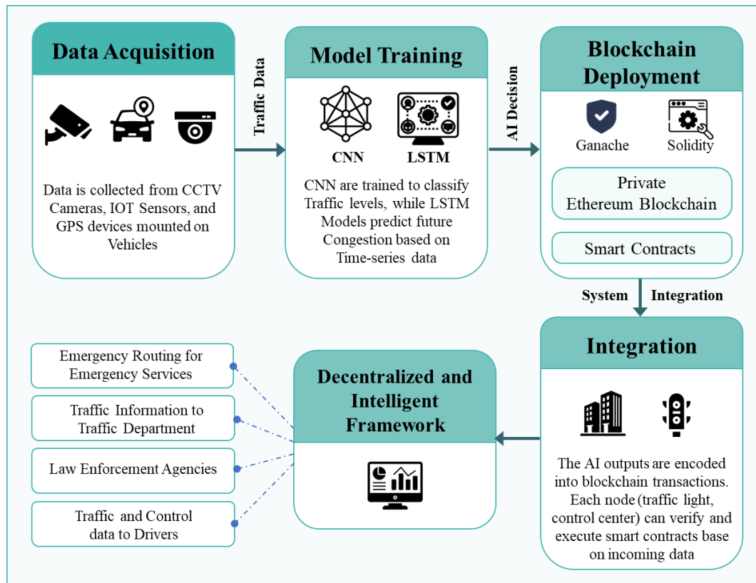
Figure 2: Intelligent Traffic Control System
