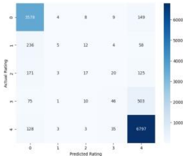
Figure 2: Confusion Matrix
