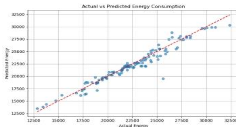
Figure 2: Actual Vs Predicted Energy Consumption
