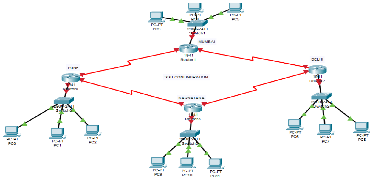
Figure 2: SSH Implementation on cisco router
