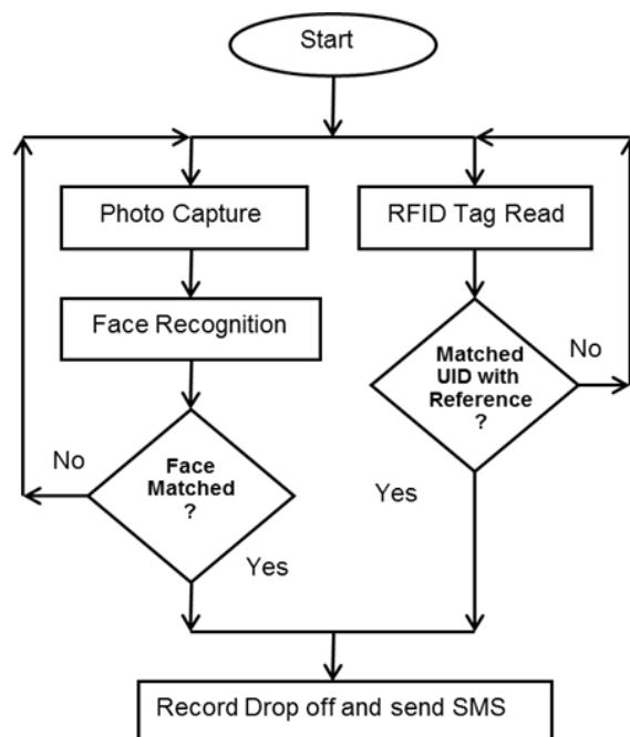
Figure 6: Flowchart of Child Drop Off Attendance System
