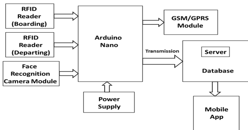
Figure 2: Hardware System Design
