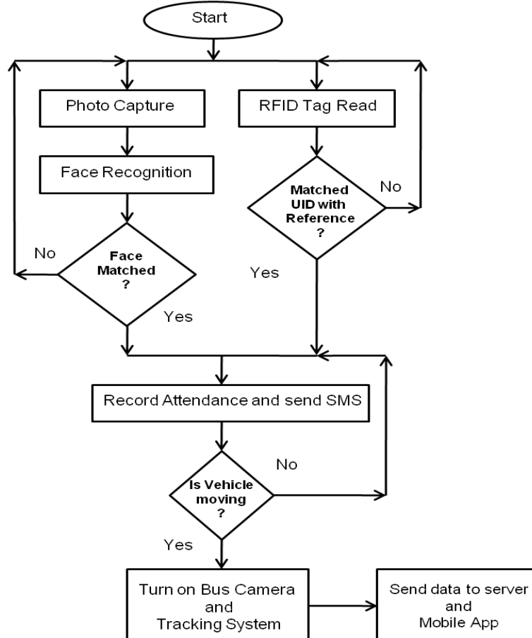
Figure 5: Flowchart of Child Boarding Attendance System
