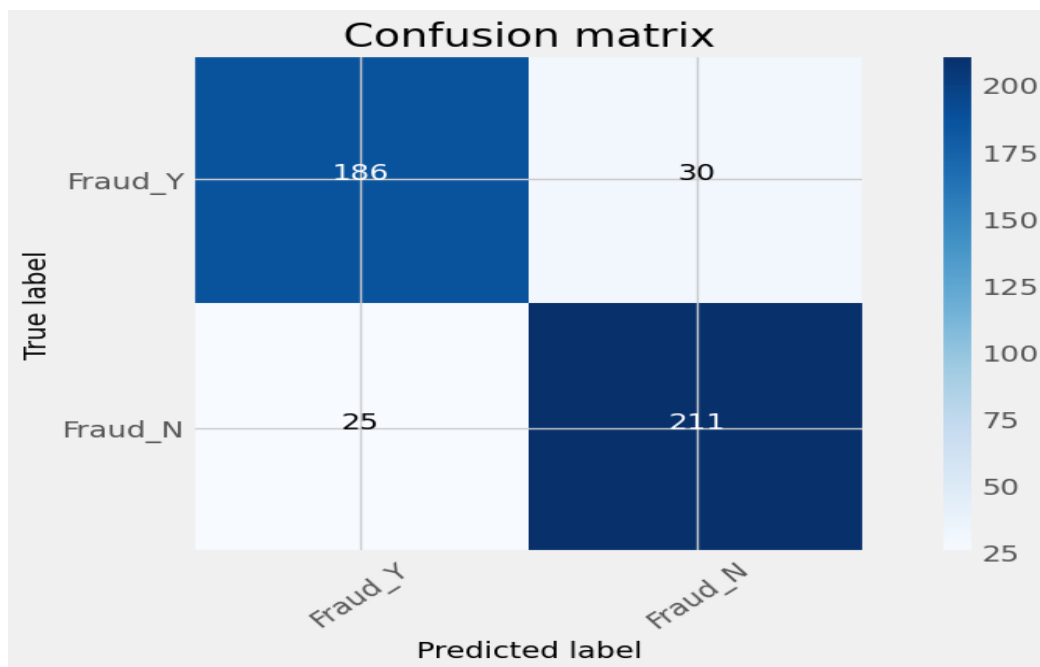
Fig 14 confusion matrix
