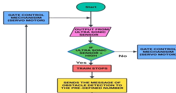
Fig 4 Flowchart for obstacle detection system
