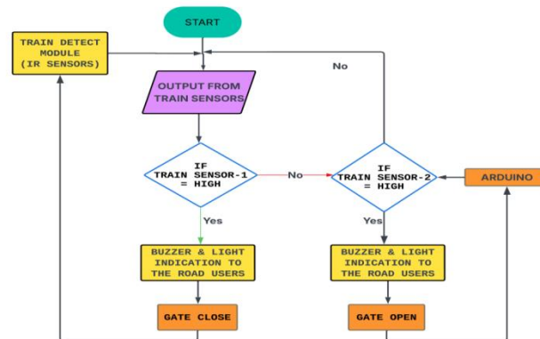
Fig 3 Flow chart for automatic railway gate control
