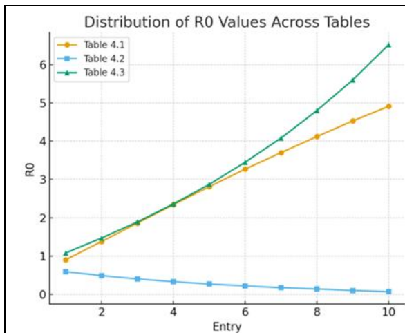
Figure 2: Distribution of R_0 values across parameter tables
