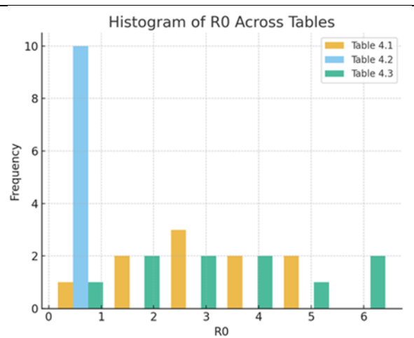
Figure 3: Histogram of R_0 across Tables 3–5
