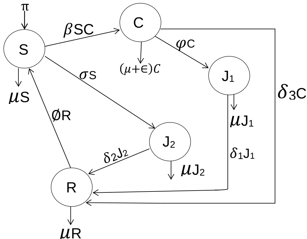
Figure 1: The flow chart of the SCJ 1 J 2 R model
