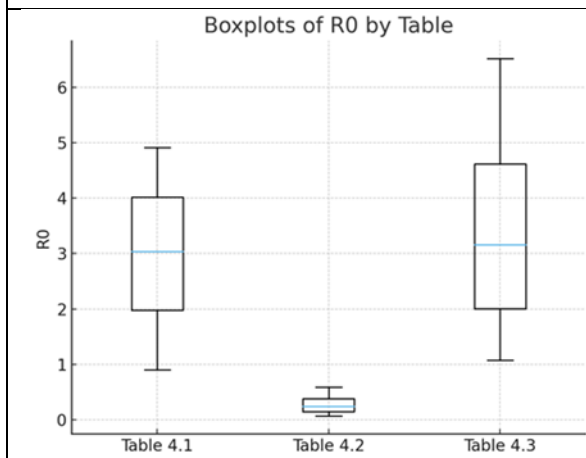
Figure 2: Distribution of R_0 values across parameter tables
