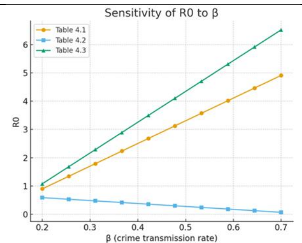
Figure 5: Sensitivity of R_0 to \beta
