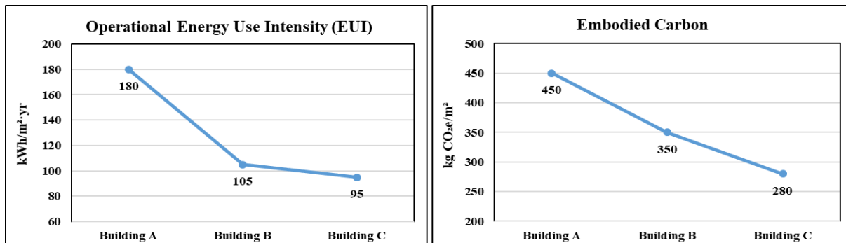
Figure 1: Comparative Data: (a) Operational Energy Use Intensity (EUI), (b) Embodied Carbon
