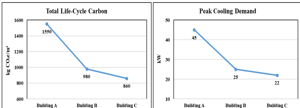
Figure 2: Comparative Data: (a) Total Life-Cycle Carbon, (b) Peak Cooling Demand
