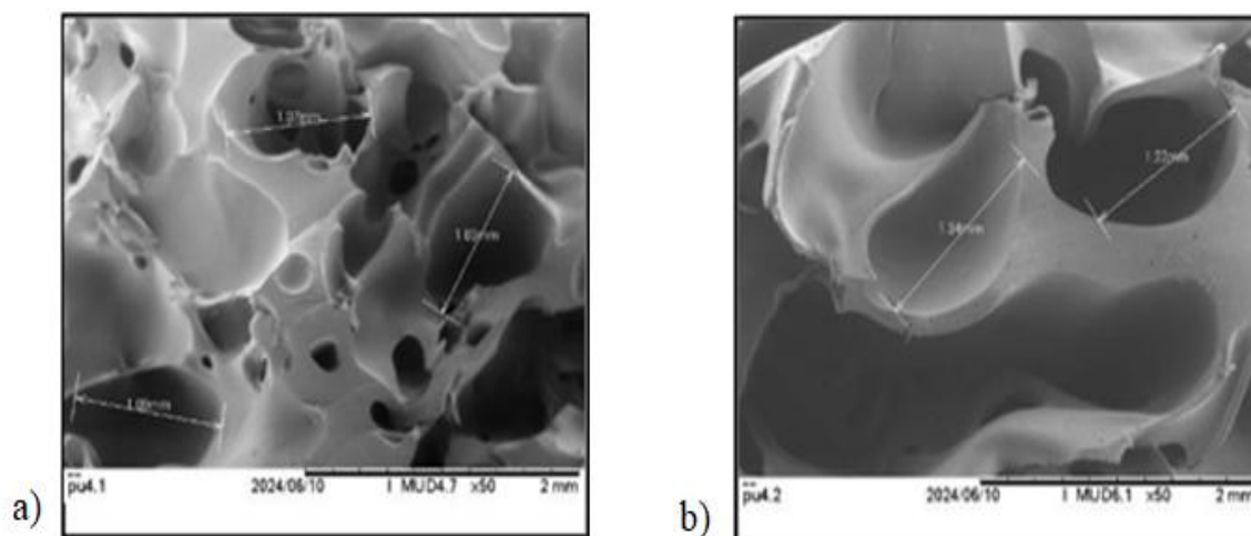
Figure 2: Average cell size of unfilled PU foam (a) without silicone oil (b) with silicone oil
