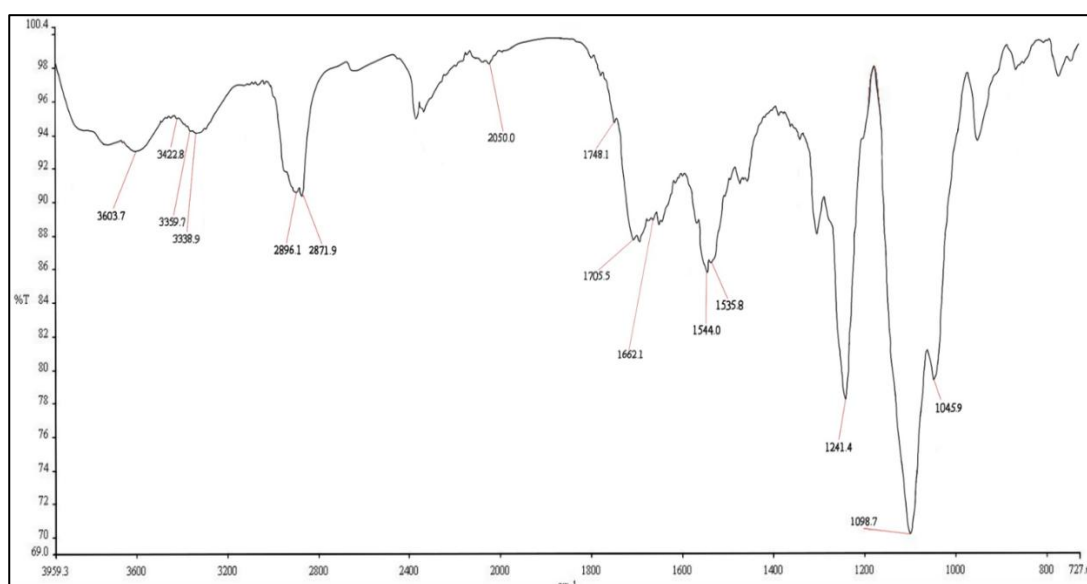
Figure 1: FTIR spectrum of synthesized PU foam
