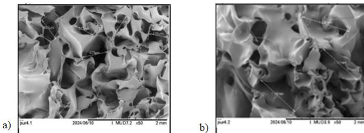
Figure 3: Average cell size of GTR-filled PU foam (a) without silicone oil (b) with silicone oil
